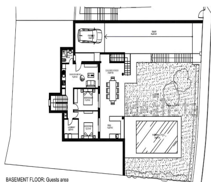
BASEMENT FLOOR: Guests area 100,00 m 2 BUILT
