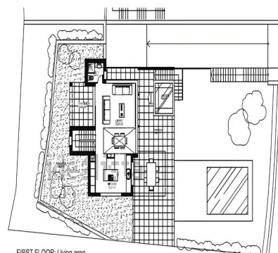
FIRST FLOOR: Living area 72,00 m 2 BUILT
